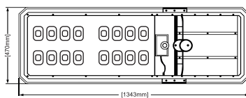
Dimension ( mm )
